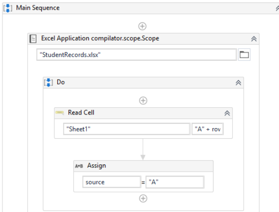
Fig. 3: A fragment of the RPA script in UIPath.
