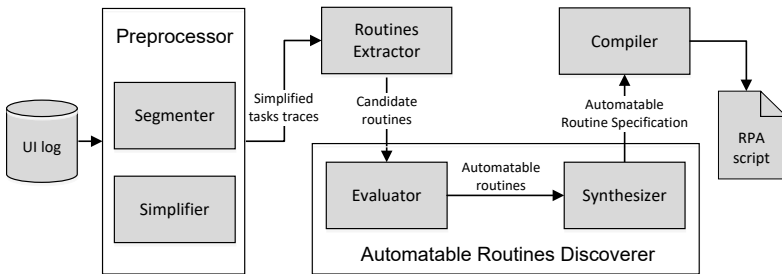
Fig. 1: Robidium architecture.
